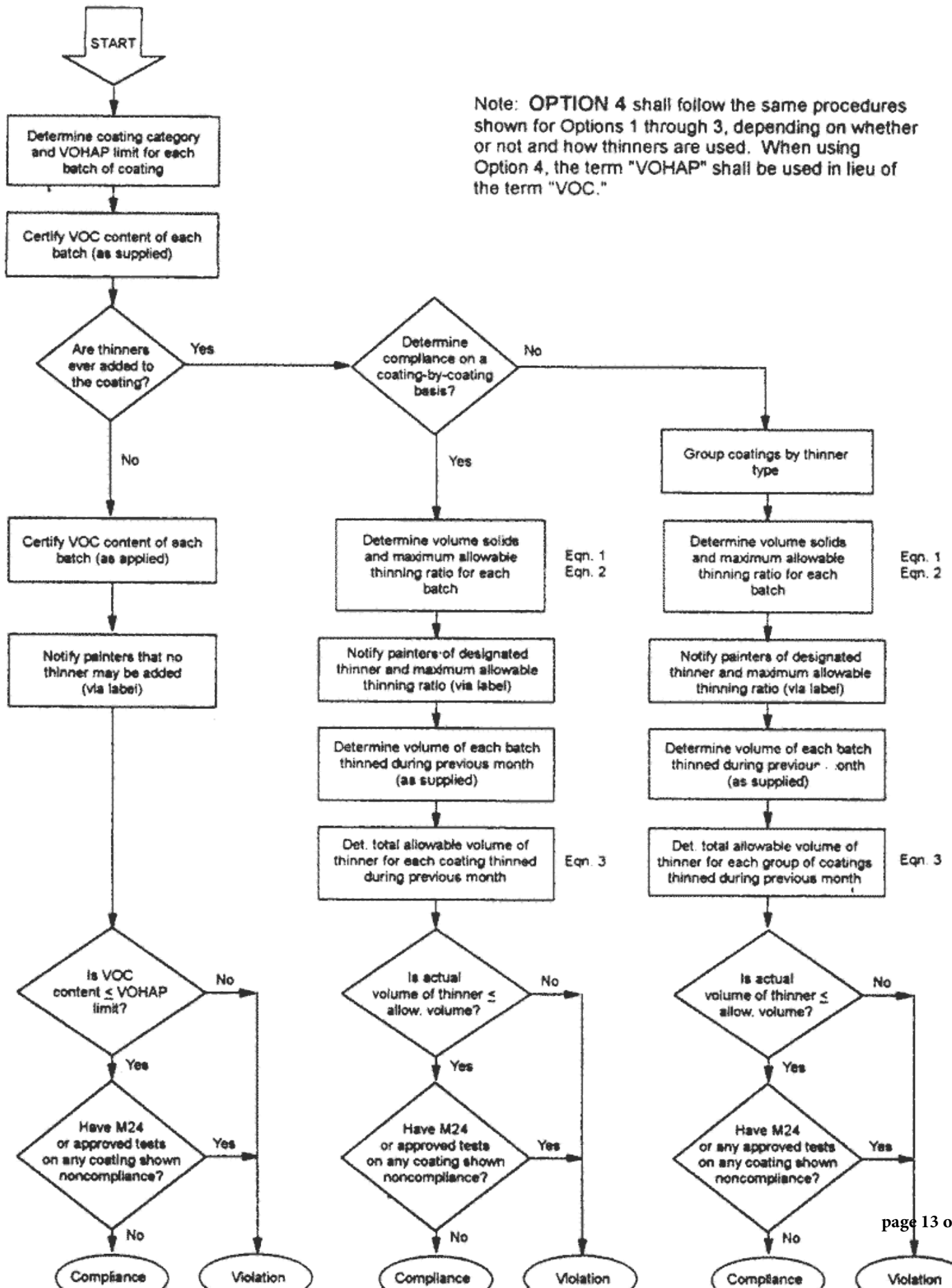
Figure 1 to §63.785 Flow diagram of compliance procedures
