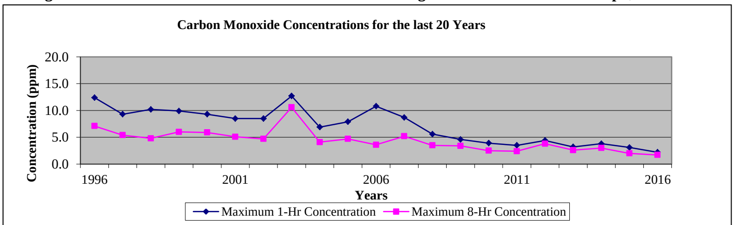
Figure 5.2 Carbon Monoxide Concentrations for San Diego-for the Last 20 Years Graph, 1996-2016
