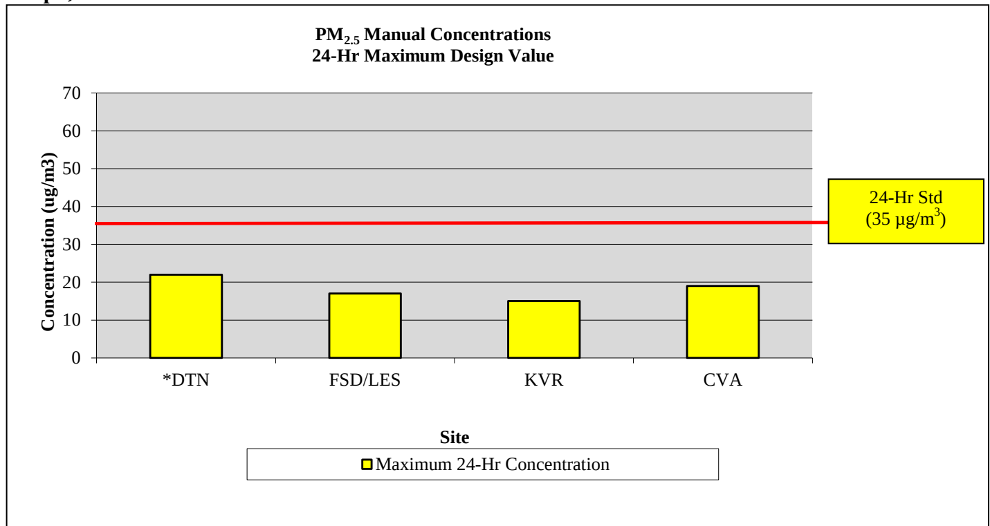
Figure 8.3a \text{PM}_{2.5} Manual Concentrations for San Diego-by Site for the Design Value (24-Hr) Graph, 2014-2016
