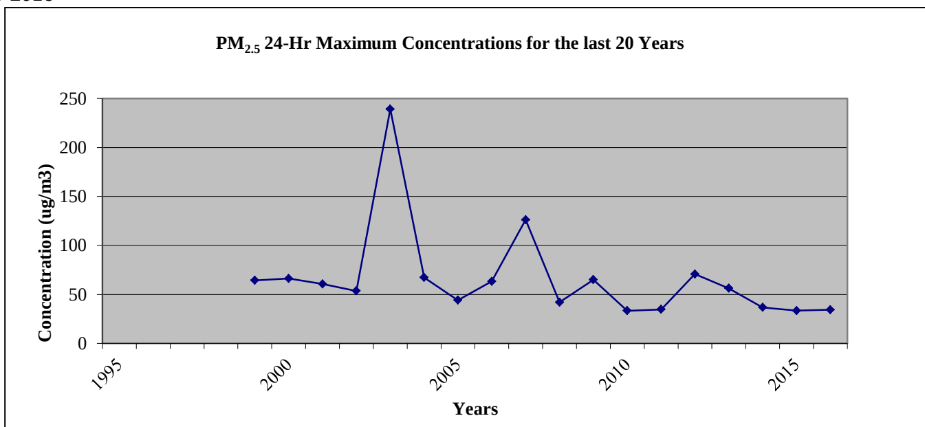
Figure 8.1 \text{PM}_{2.5} Manual Concentrations for San Diego-for the Last 20 Years (24-Hr) Graph, 1996-2016
