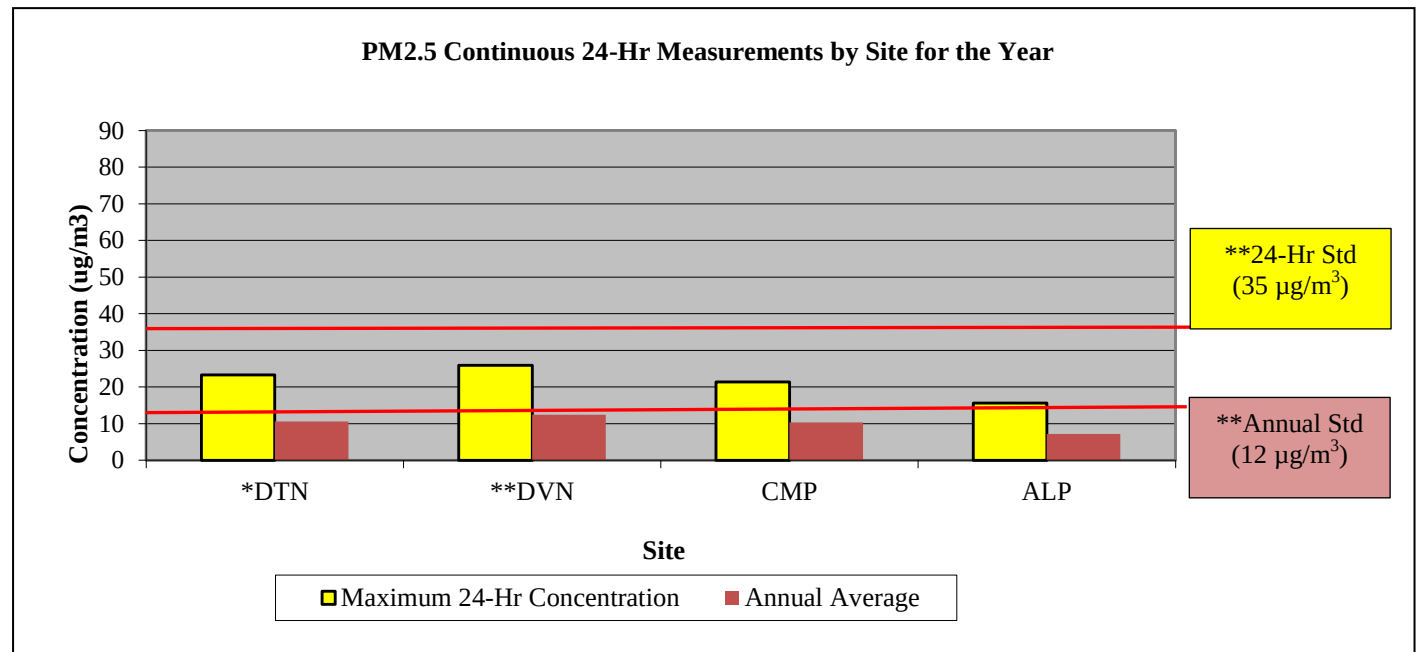
Figure 8.5 \text{PM}_{2.5} Continuous Concentrations for San Diego-by Site for the Design Value (24-Hr & Annual Average) Graph, 2014-2016
