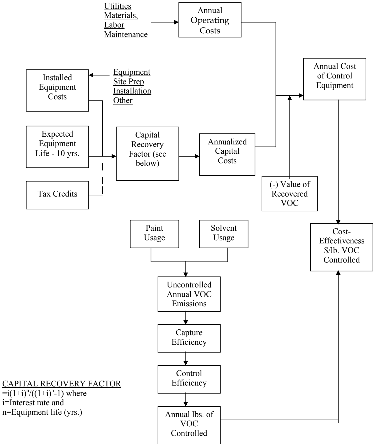
FIGURE 2.5 BACT COST-EFFECTIVENESS PROCESS FLOWCHART
