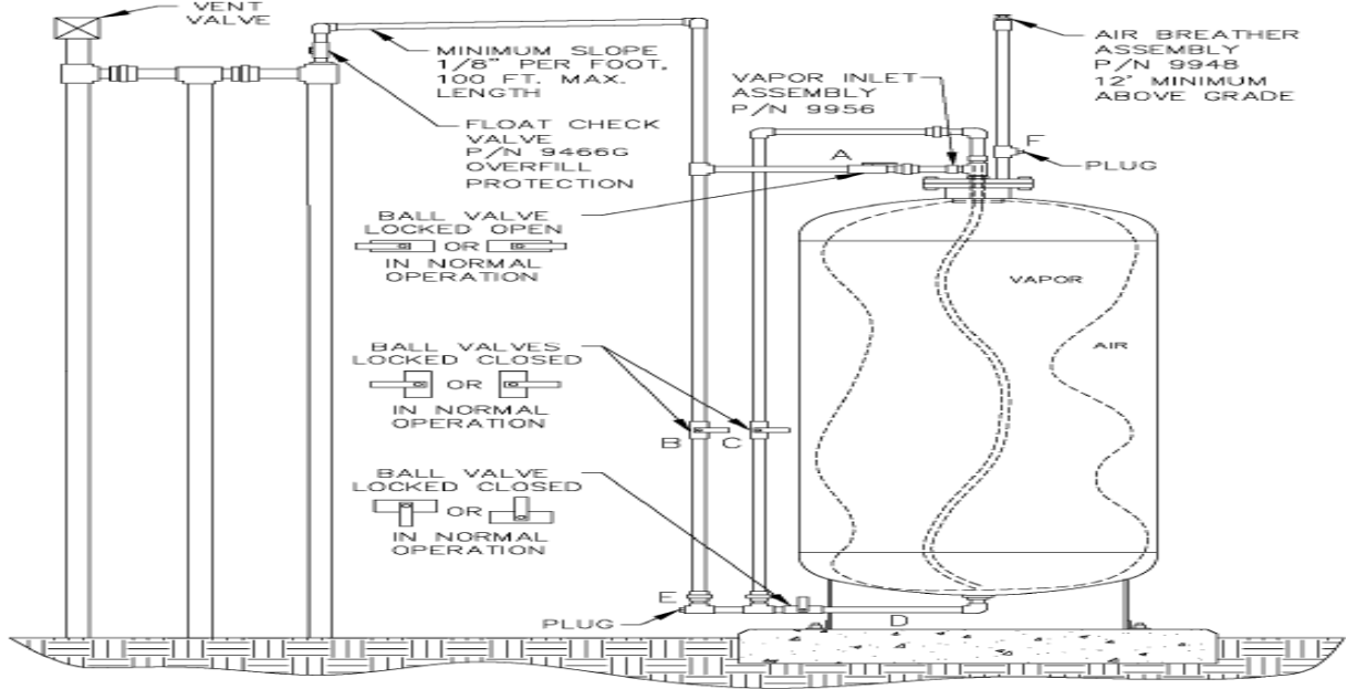
Clean Air Separator Normal Operating Configuration
